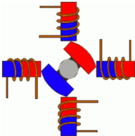
Two-Coil excitation
